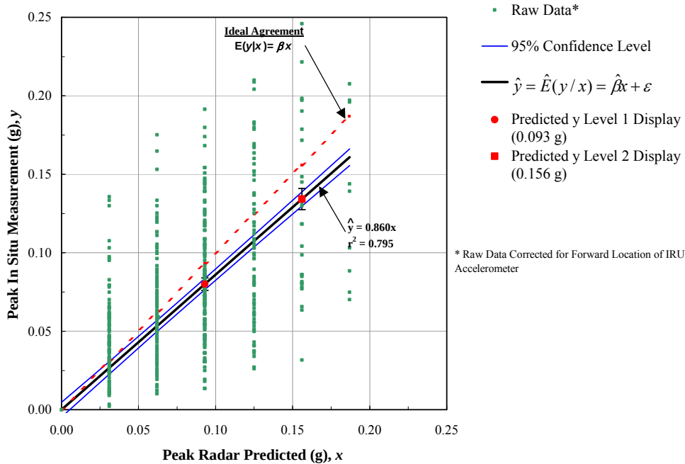
Figure 46: Correlation of Radar Predicted & In Situ Peak \sigma_{An}
